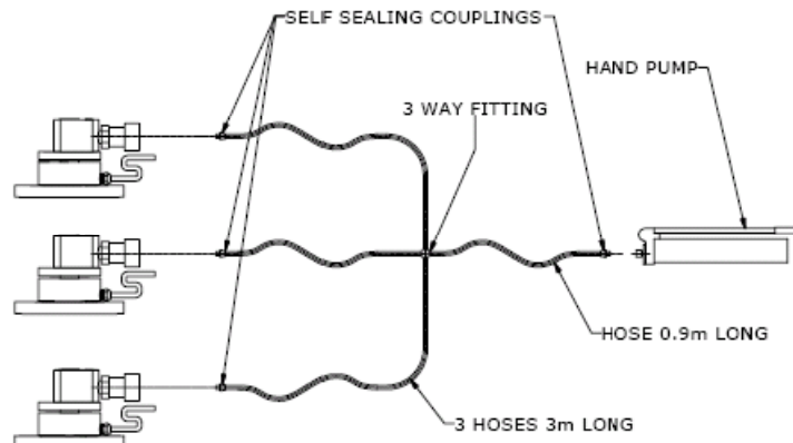
(3 Static Compression cell System)
